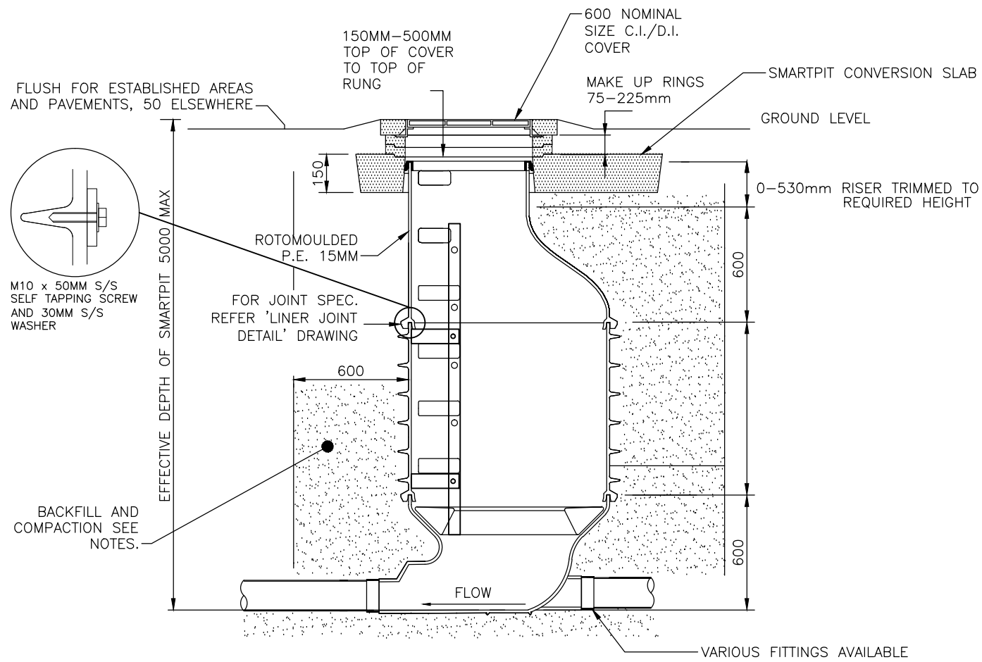
SECTION 'A-A'
